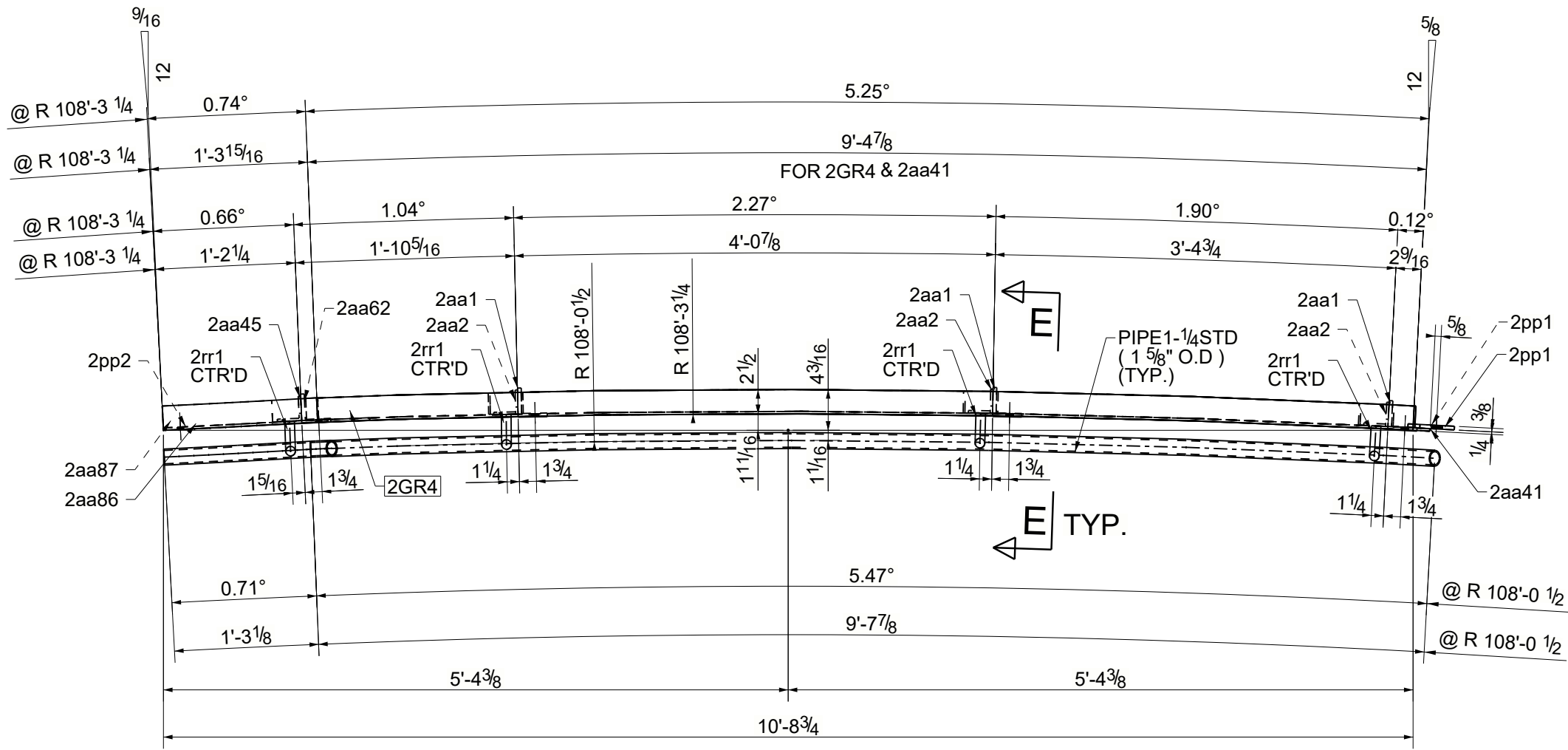
A-A PLAN VIEW
