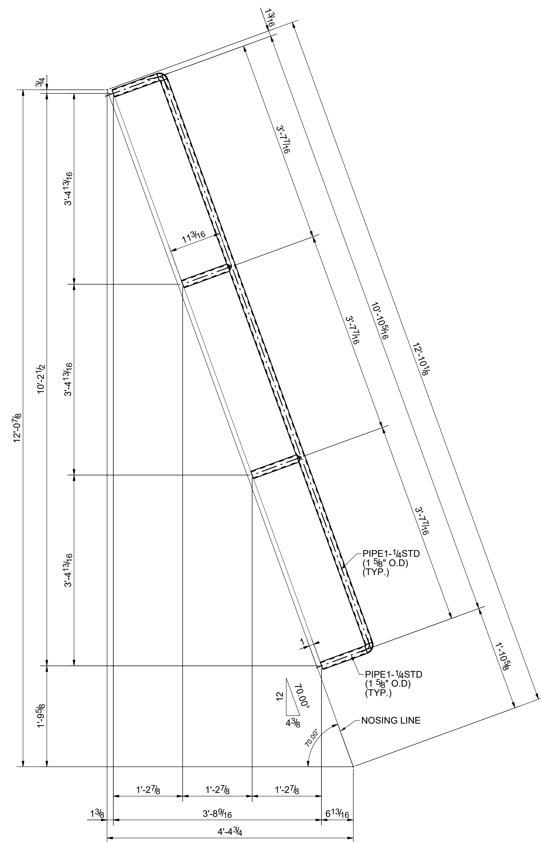
DETAIL 1
