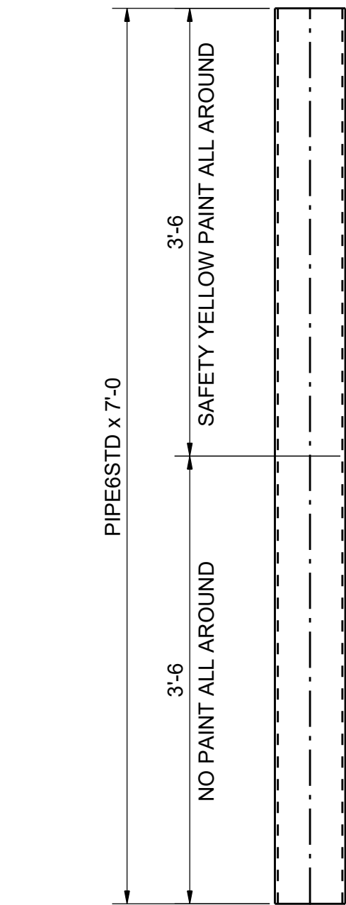
25 - BOLLARDS - M240M1
