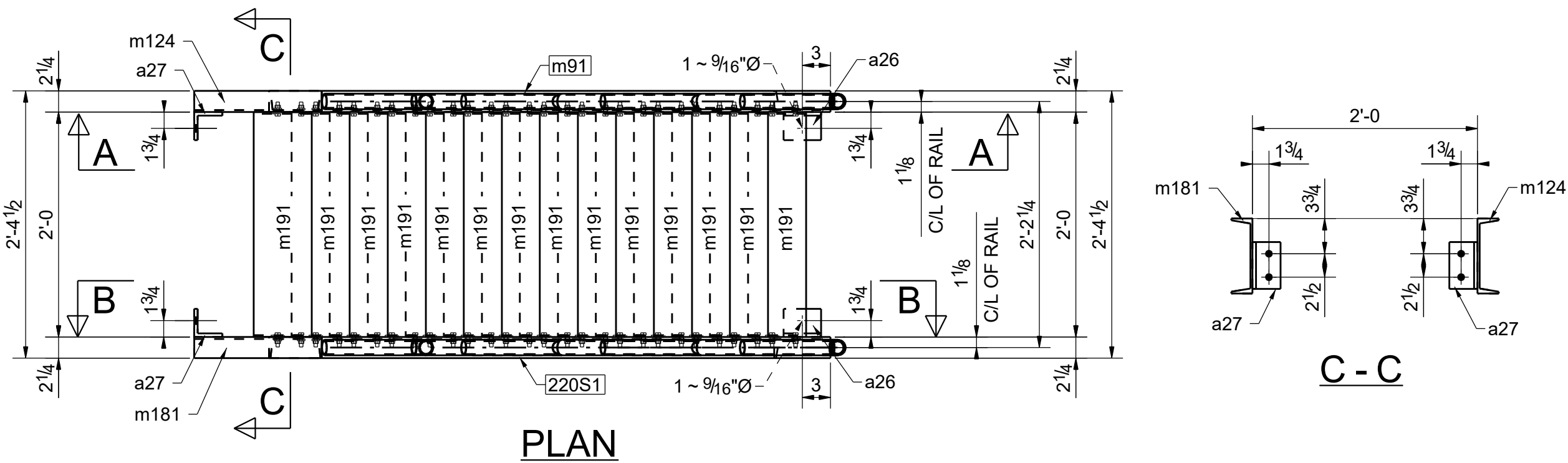
ONE - SHIP LADDER - 220S1
