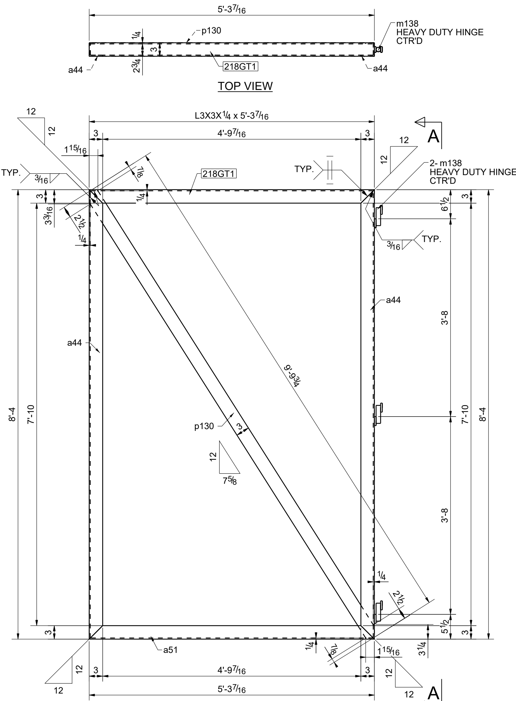
ONE - GATE FRAME - 218GT1
