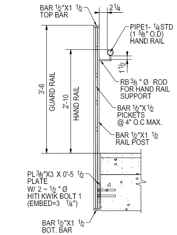
1 - 1 TYPICAL STAIR RAIL DETAIL
