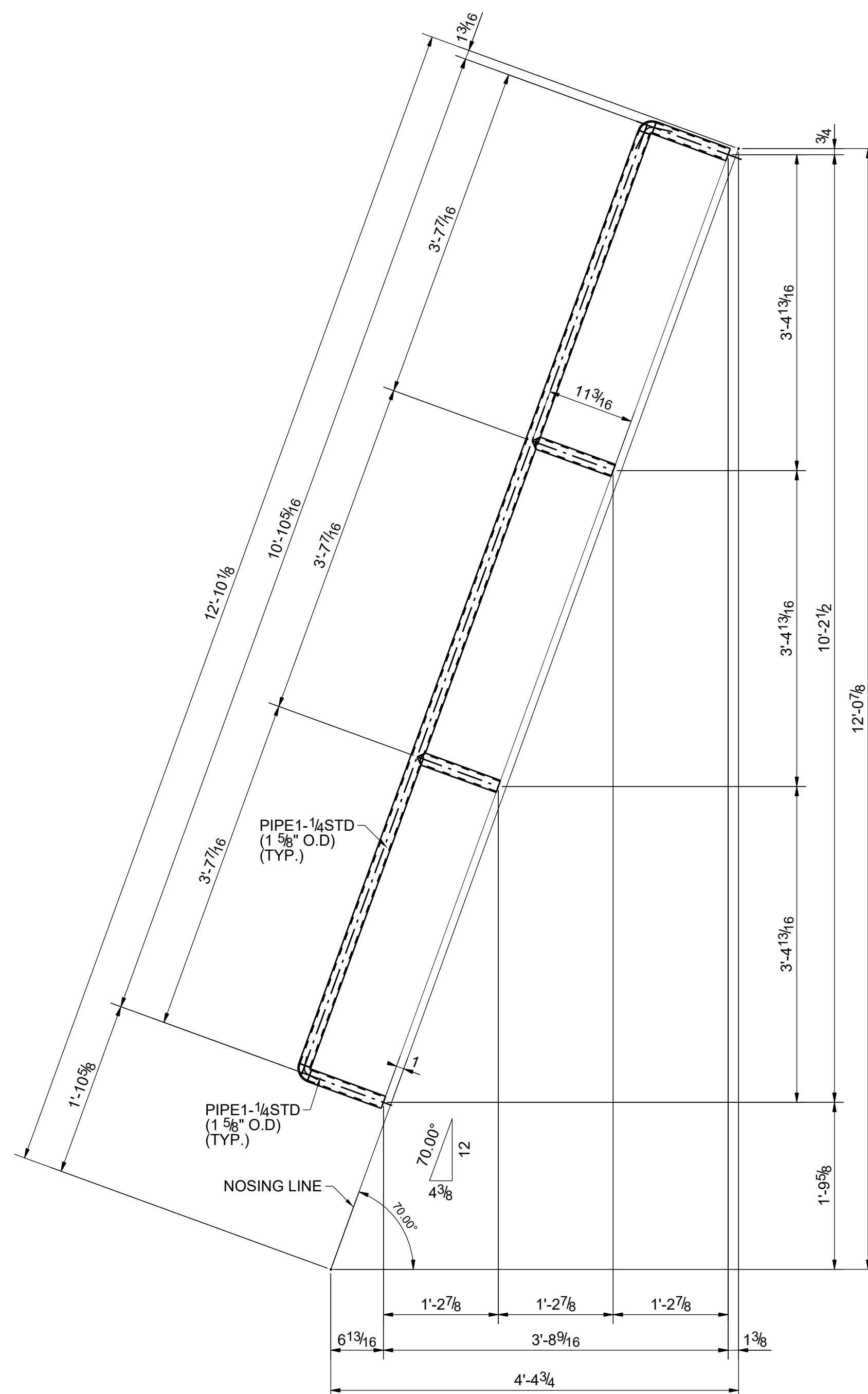
DETAIL 2
