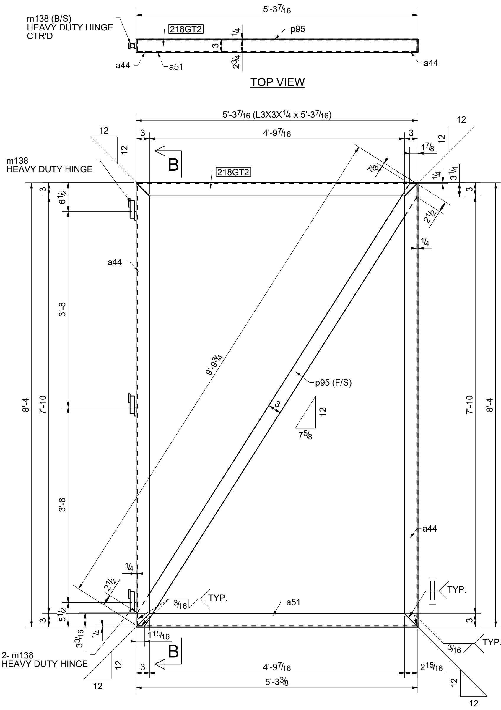
ONE - GATE FRAME - 218GT2
