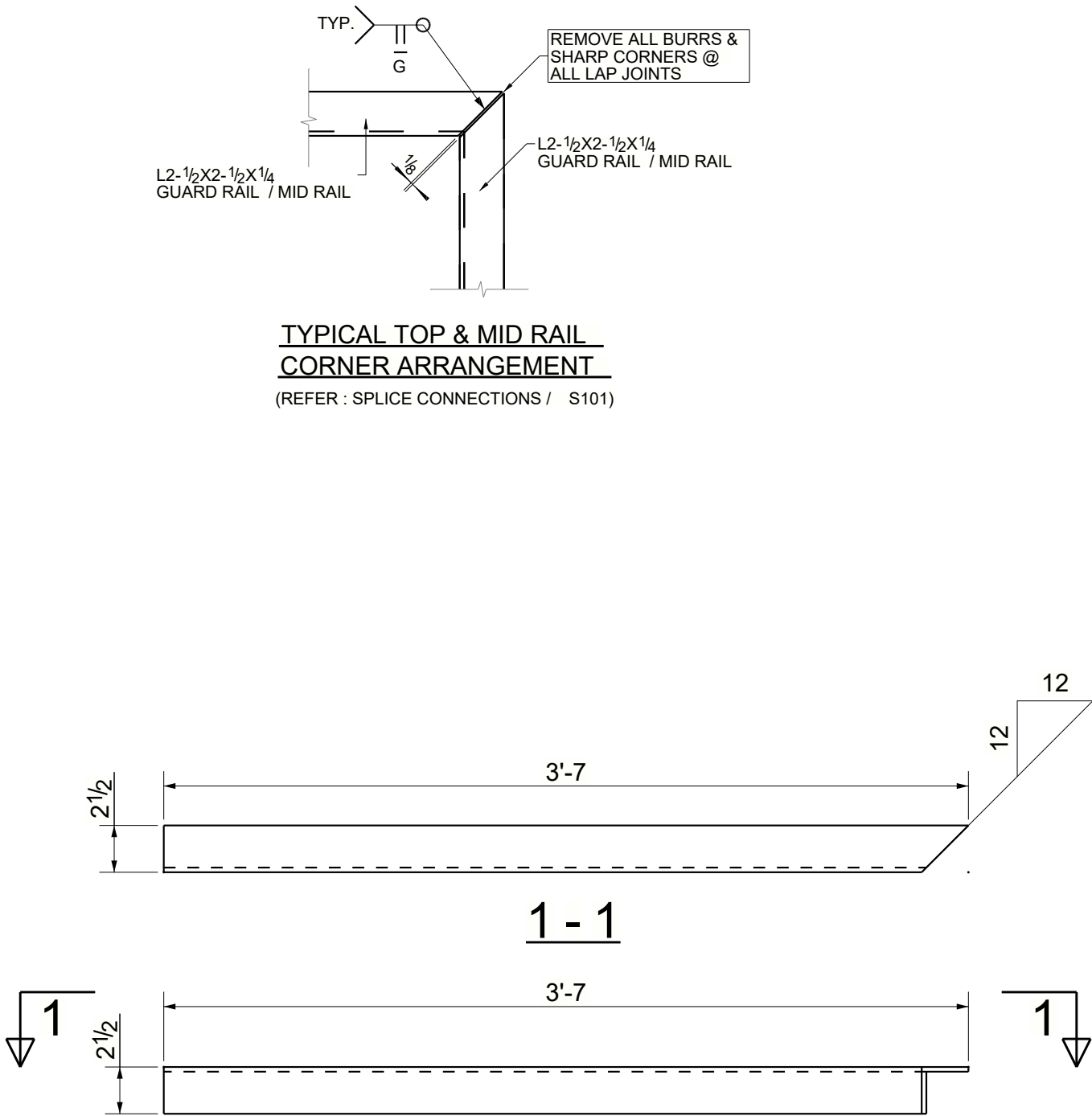
DETAIL OF GR21
