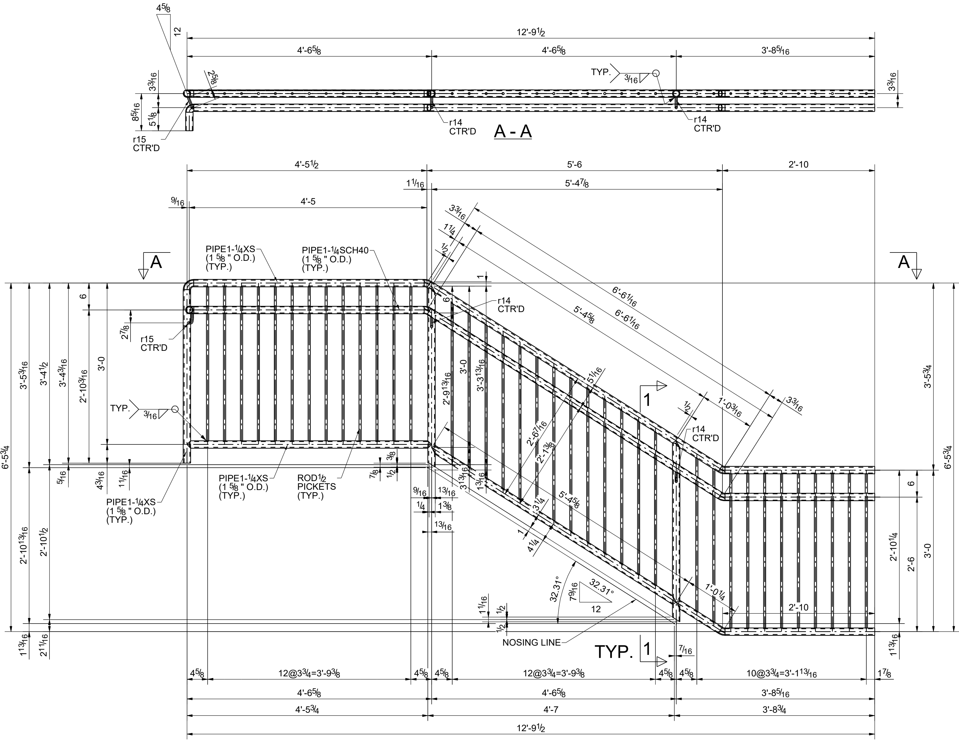
ONE - GUARD RAIL - M224GR1
