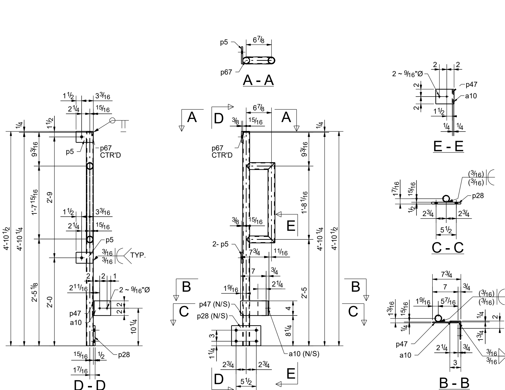
2 - HANDRAILS - 121HR1
