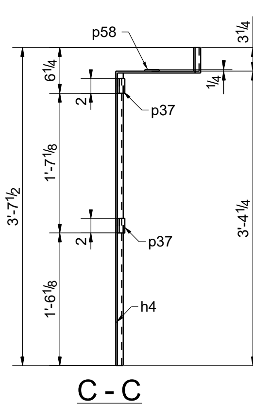
DETAIL OF 104F1
