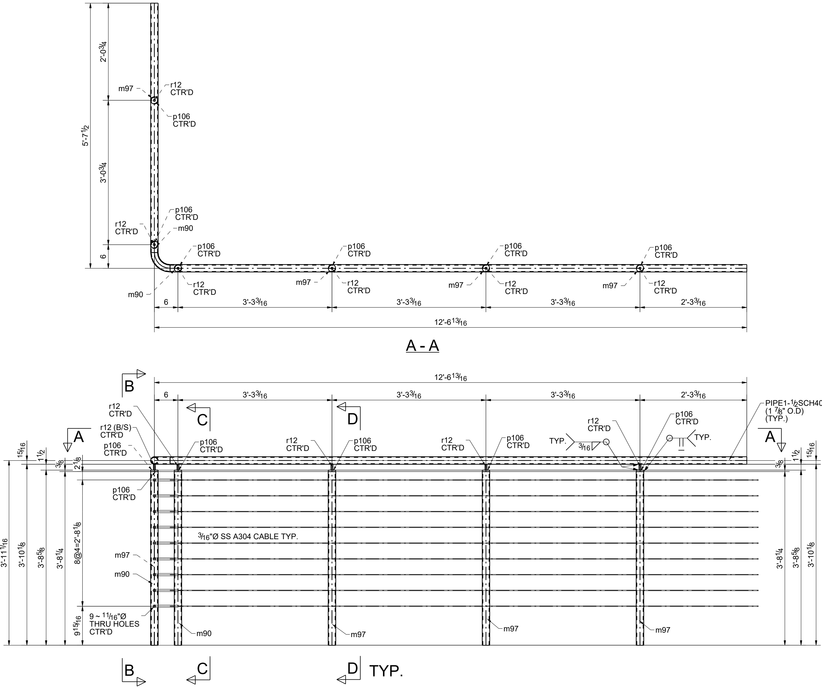
ONE - GUARD RAIL - M242GR1
