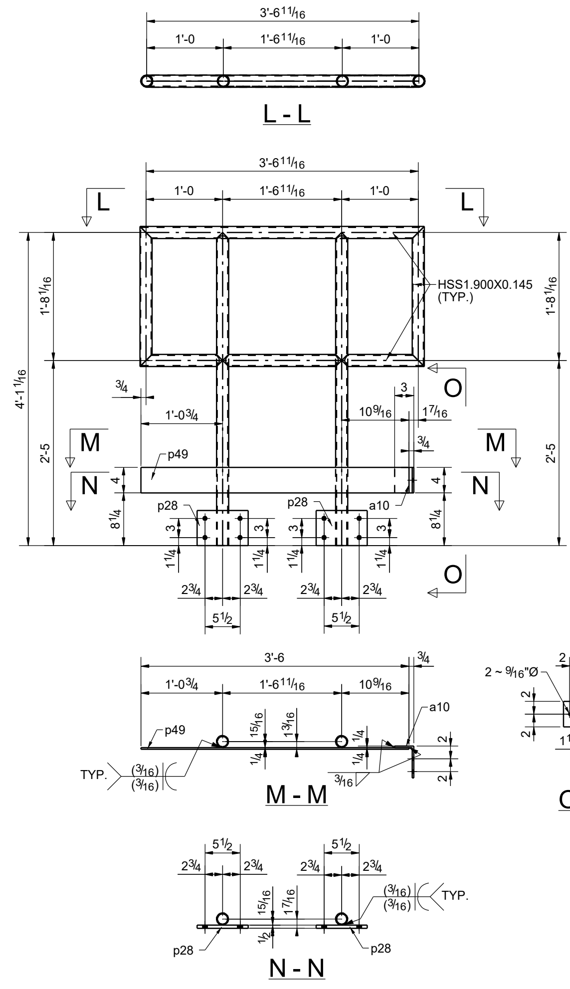
ONE - HANDRAIL - 121HR4
