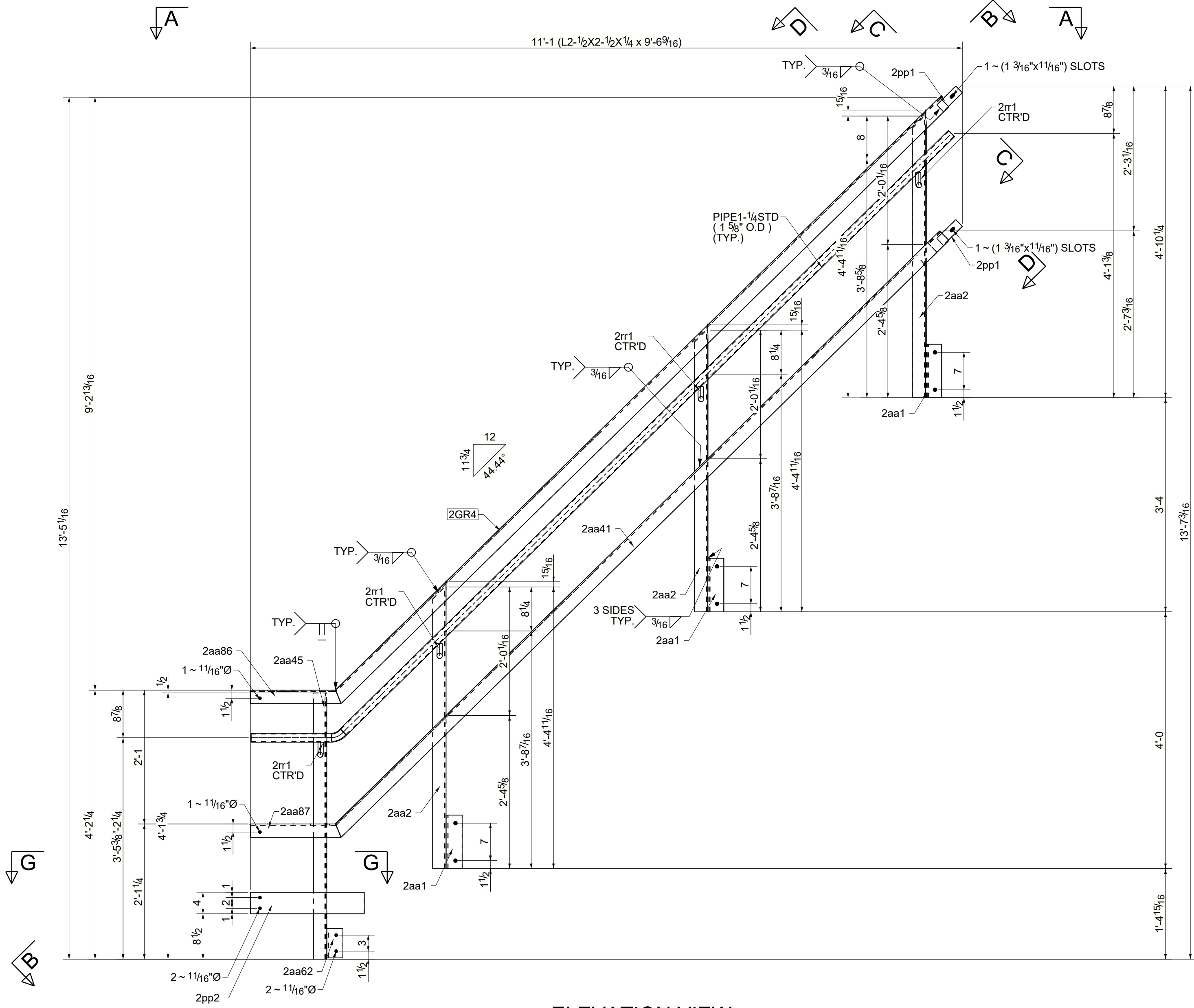
ELEVATION VIEW
