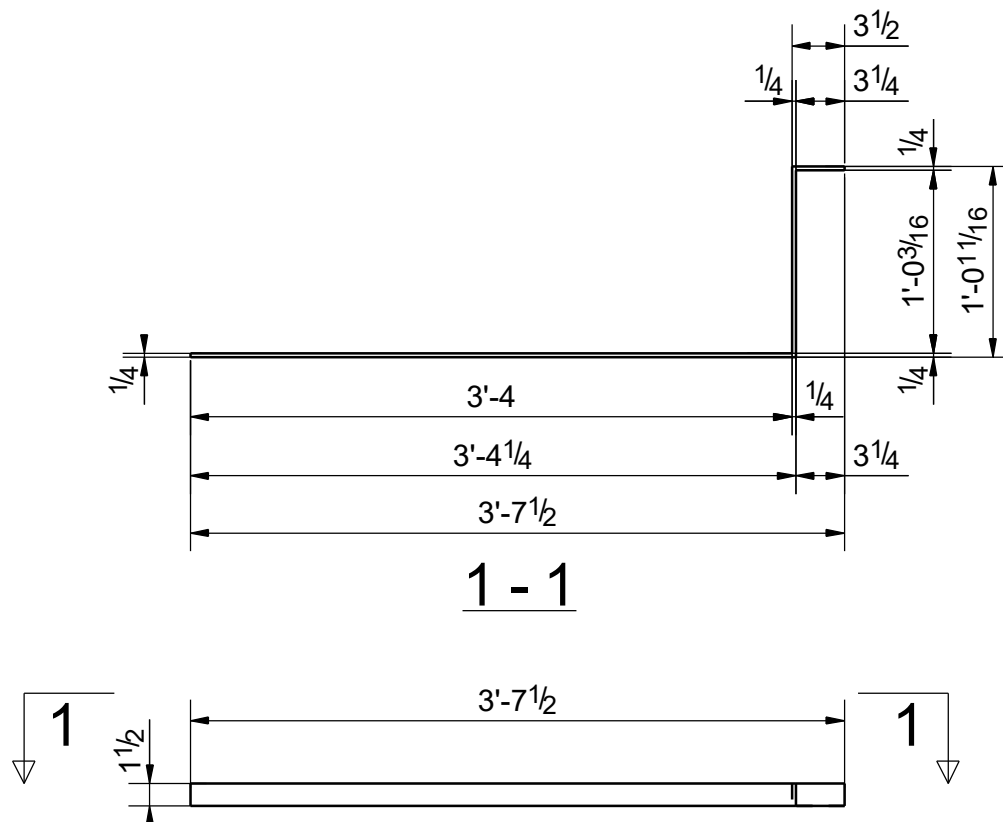
DETAIL OF 104F1
