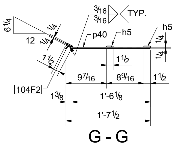
ONE - FRAME - 104F2
