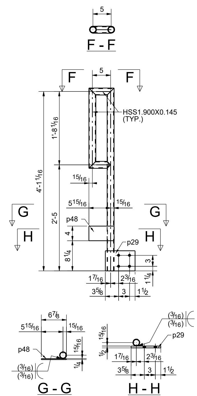
2 - HANDRAILS - 121HR2
