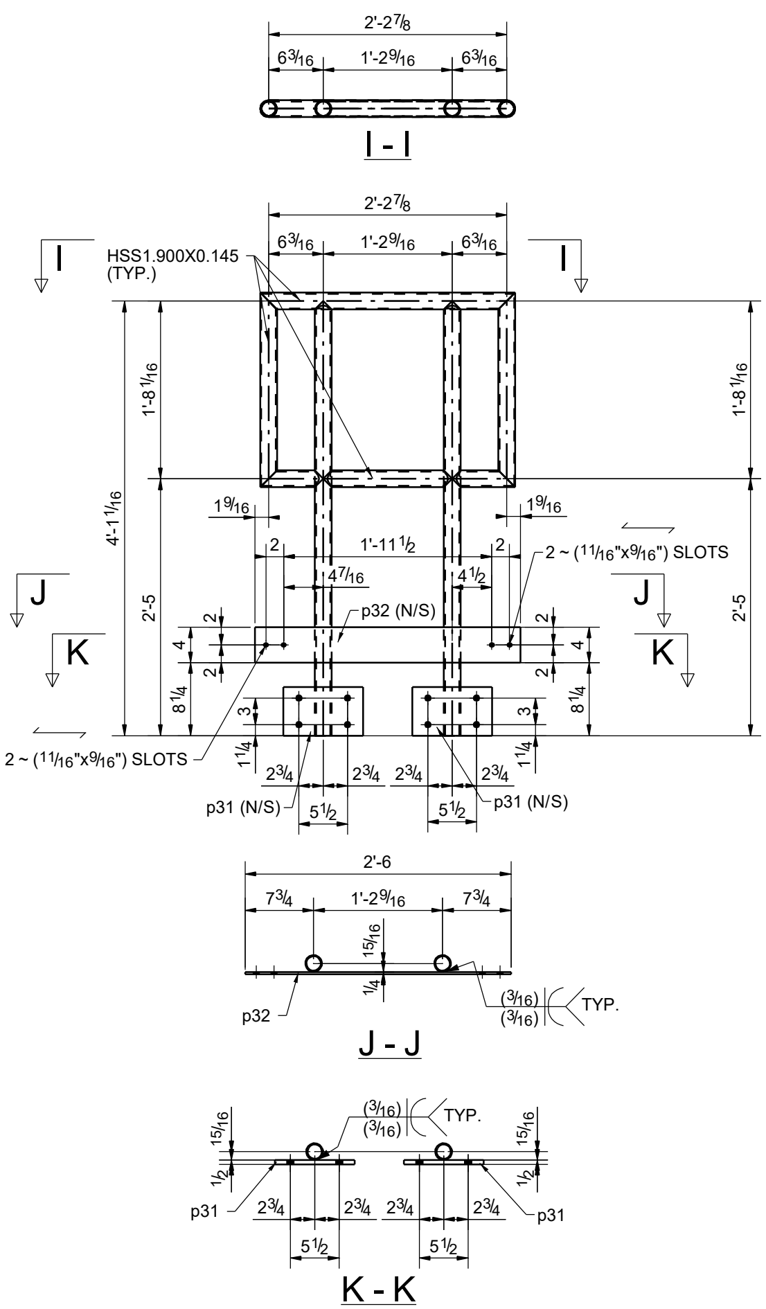
ONE - HANDRAIL - 121HR3
