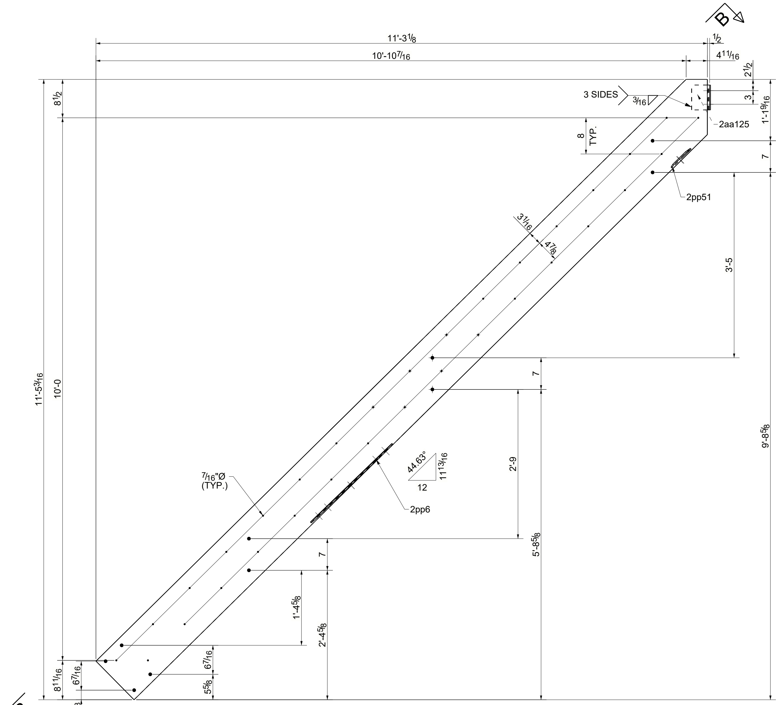
A - A ELEVATION VIEW
